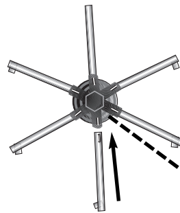
Illus. 1 Cupola Top Poles inserted into Center Hub
